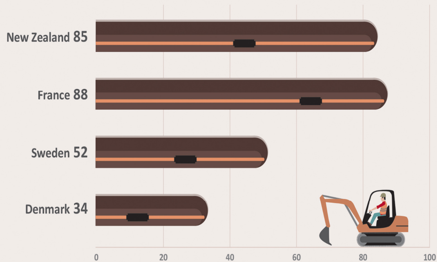
Average trenching cost (investment NZD/metre)
