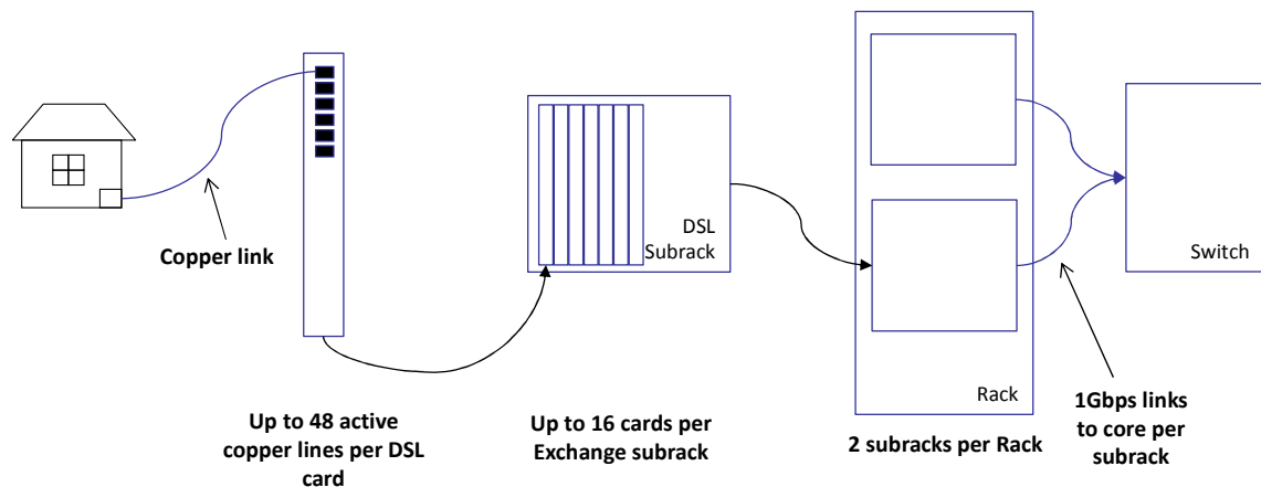
Figure 36 – DSLAMs dimensioning
