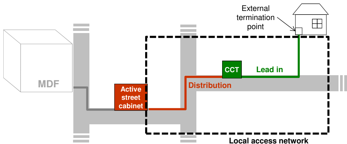
Figure 23 – Architecture of the local access network when the street cabinet is active
