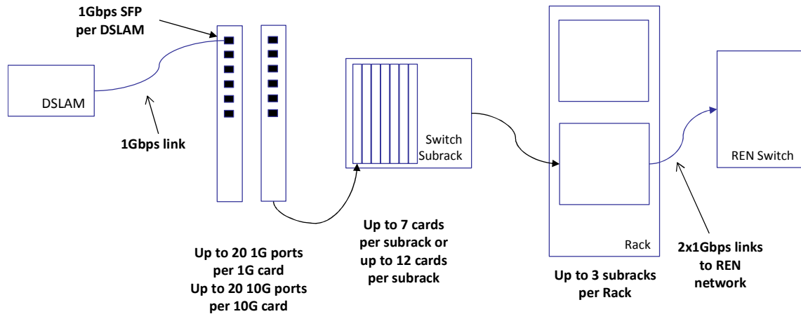
Figure 37 – FDS dimensioning
