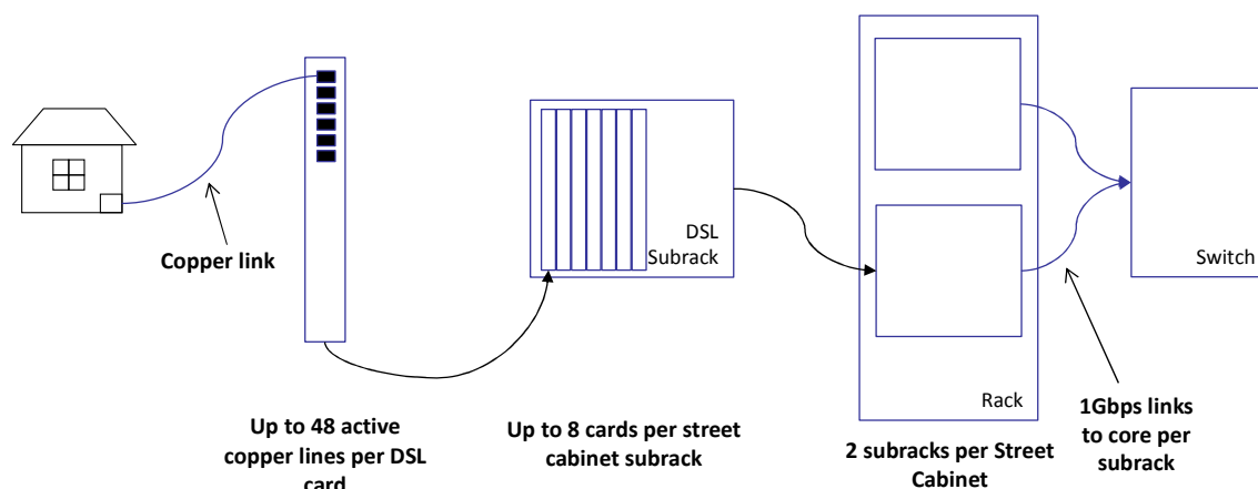
Figure 35 – DSLAMs dimensioning
