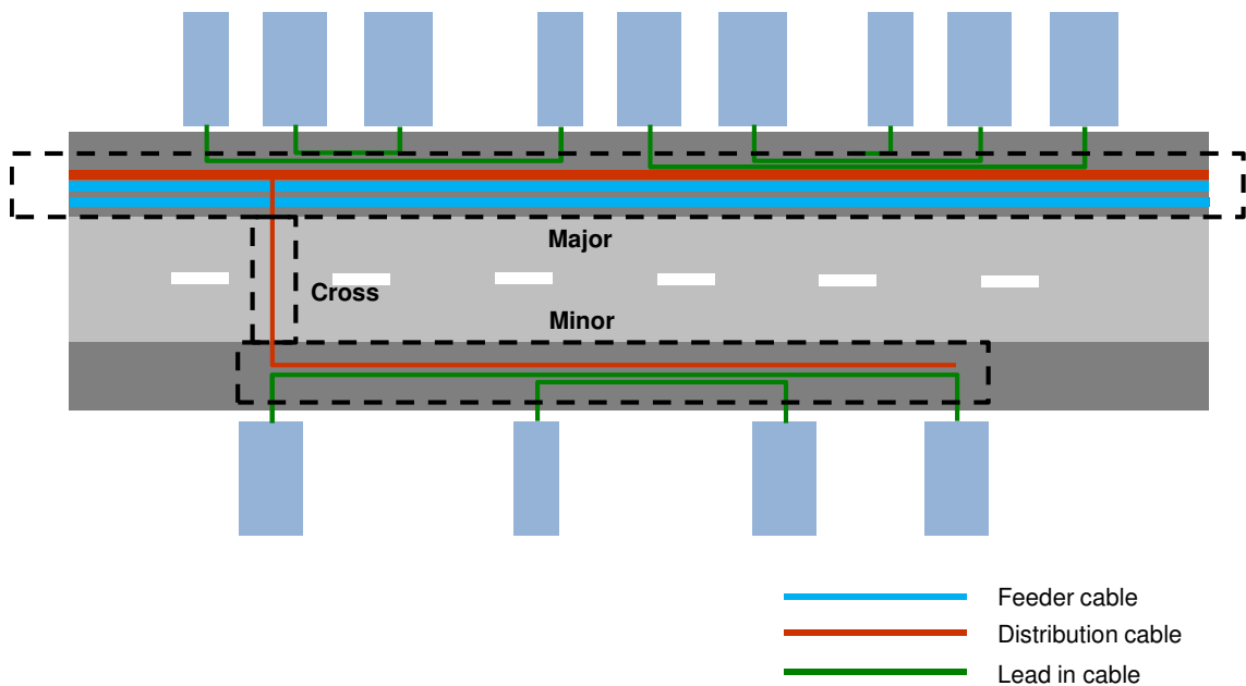
Figure 29 – Horizontal trenches
